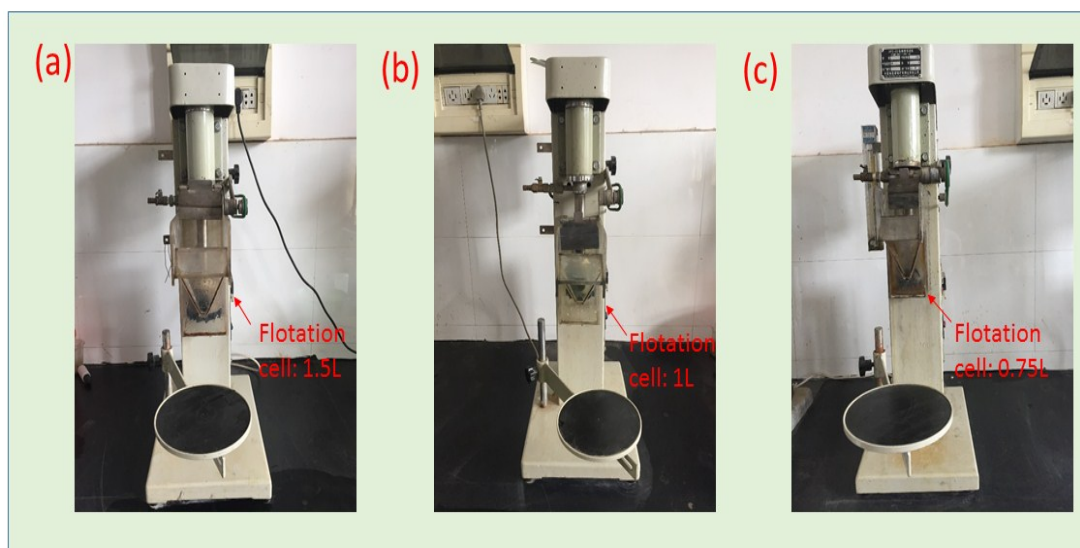
Figure S1. The photo images of flotation machine which are (a) handling capacity of 1.5 L, (b) handling capacity of 1 L and (c) handling capacity of 0.75 L.
