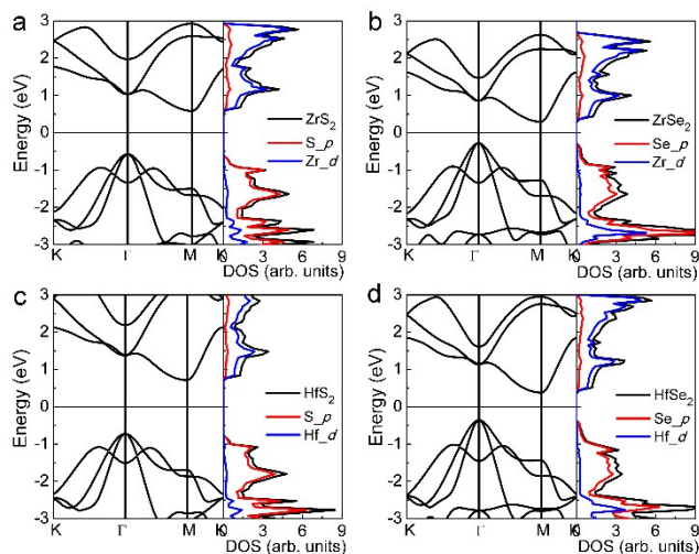
Fig. S1 The band structures and DOS of MX 2 (M=Zr, Hf; X=S, Se) monolayers. The red and blue lines in the right image represent the contribution of the p orbital of the S (Se) atoms and the d orbital of the Zr (Hf) atoms, respectively.
