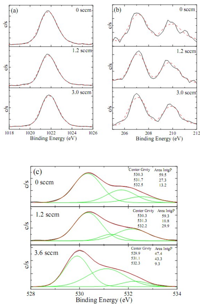
Fig. 4. The typical XPS spectra of (a) Zn 2p, (b) Nb 3d, and (c) O 1s of the NZO films with and without H doping.
