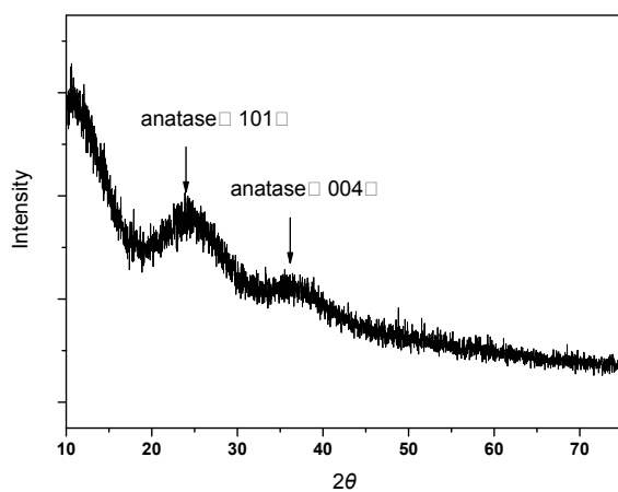
Fig. S1 The XRD results of the gel, indicating the amorphous nature.
