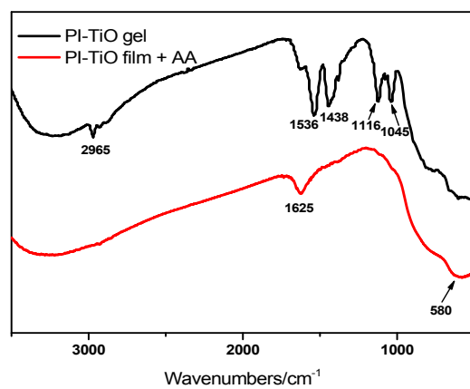
Fig. S5 The FTIR spectrum of the PI-TiO gel and PI-TiO film after binding with AA.
