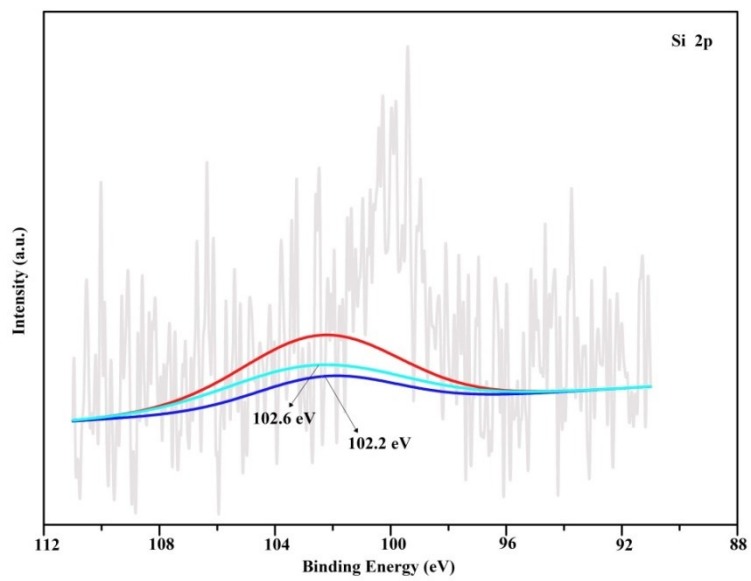
Fig. S1 Si 2p XPS spectra of GOF dispersions.
