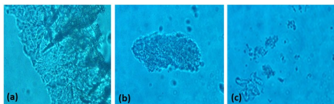
Figure S2. Images obtained from three different regions after 45 minutes RBC exposure to ~ 390 µg/ml BPA
