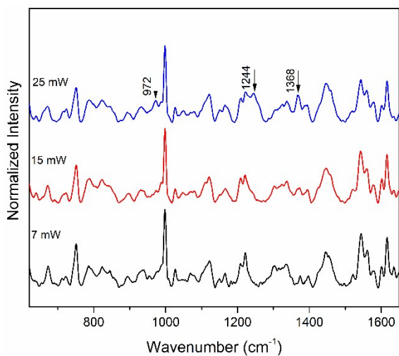
Figure S1. Laser power dependent study on RBC. Heme aggregation markers are highlighted by arrows in the figure
