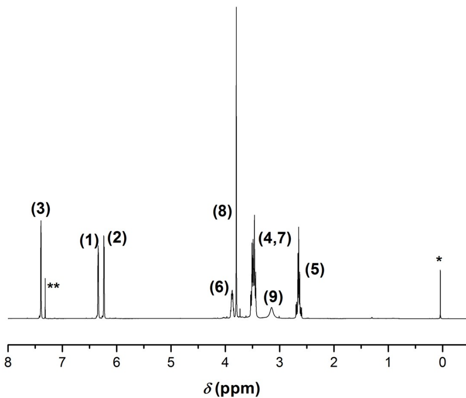
Figure S2. The liquid 1 H NMR spectrum of Tetra Furan (* denotes the TMS signal peak, ** denotes the solvent signal peak)
