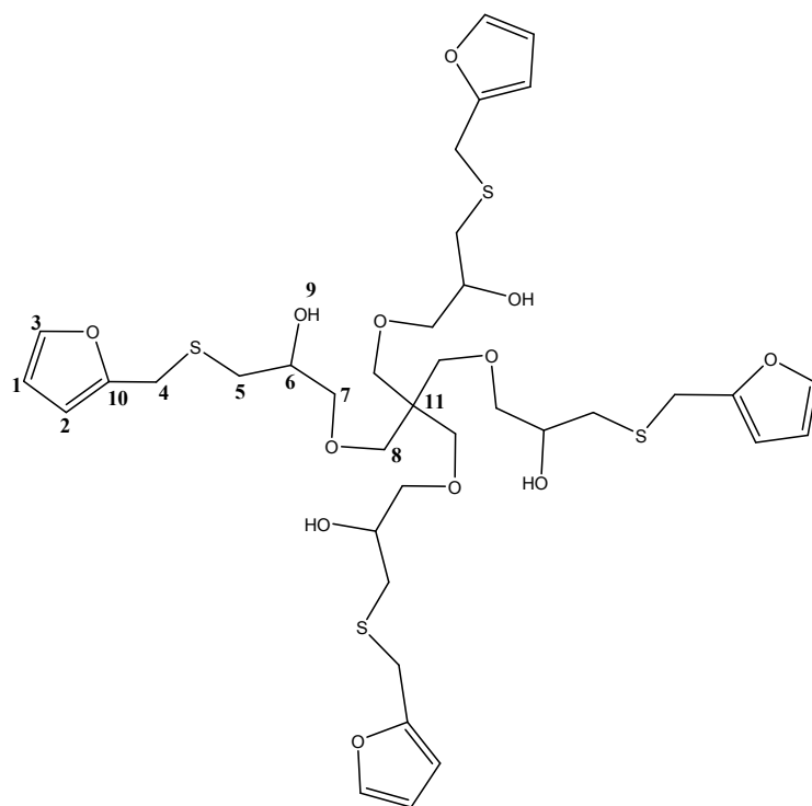
Figure S1. The structure of Tetra Furan
