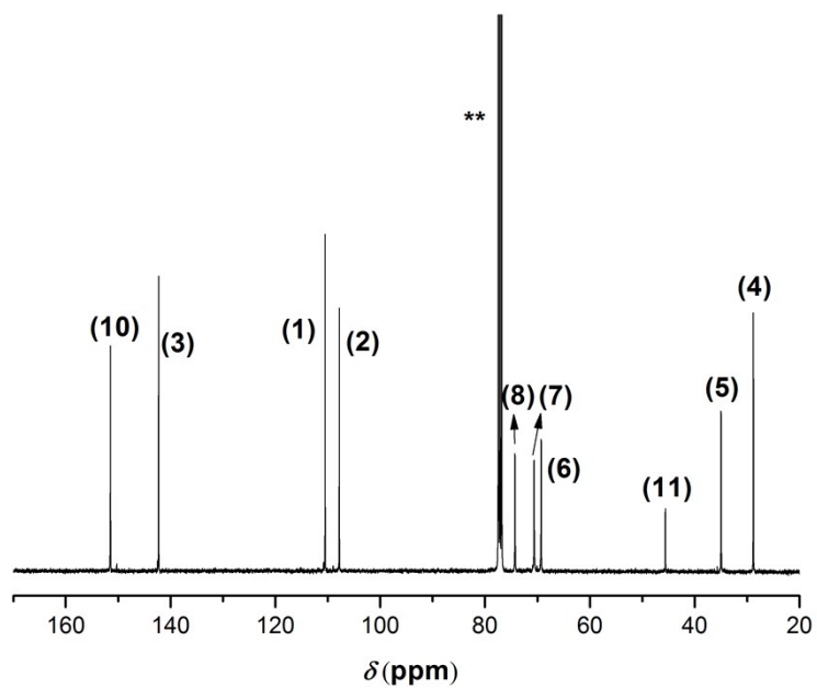
Figure S3. The liquid ^{13}\text{C} NMR spectrum of Tetra Furan (** denotes the solvent signal peak)
