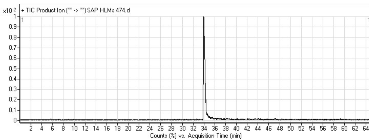
Fig. S1. SAP PI chromatogram. SAP, sapitinib; PI, product ion.
