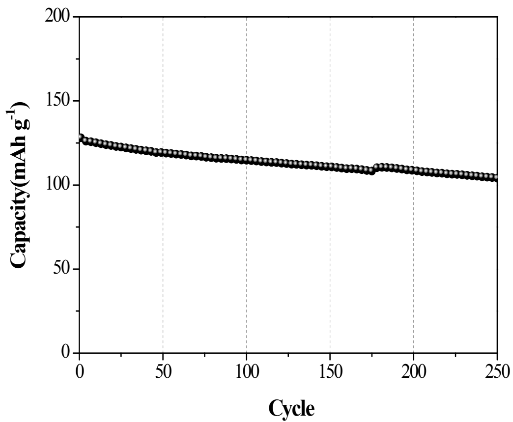
Fig. S2 Cycle performance of the nanosized LMO/C sample prepared by pyro synthesis at 1C current density in the voltage range 3.0 to 4.3 V.
