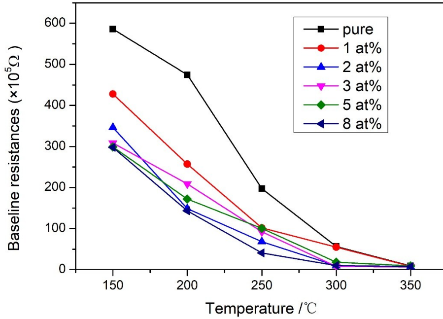
Figure. S3. The baseline resistances curve of the sensors based on pure WO 3 , 1 at%, 2 at%, 3 at%, 5 at% and 8 at% Pd-WO 3 at different working temperature toward 100 ppm acetone
