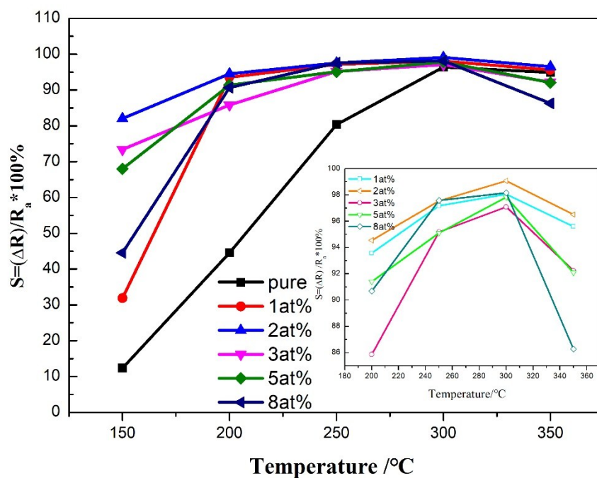
Figure. S1. Responses ( S = (\Delta R/R_a) * 100\% ) curve of the sensors based on pure WO_3 , 1 at%, 2 at%, 3 at%, 5 at% and 8 at% Pd- WO_3 at different working temperature toward 100 ppm acetone.
