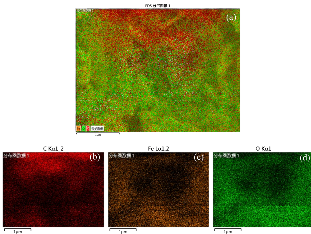
Fig. S2 The EDS elemental mapping of (a) all elements, (b) C, (c) Fe, and (d) O elements of the BC-nZVI sample
