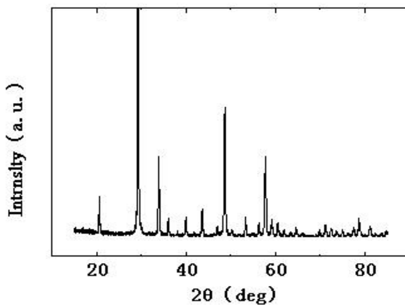
Fig. S2 XRD pattern of Y_2O_3 NPs
