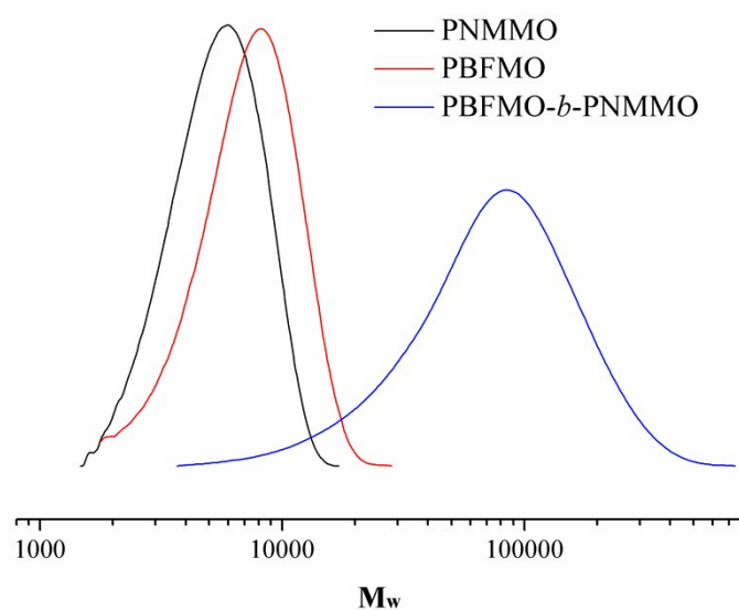
Fig. S1. GPC curves of PNMMO ( M_n=4650 \text{ g mol}^{-1} , PDI=1.18), PBFMO ( M_n= 6840 \text{ g mol}^{-1} , PDI=1.22) and PBFMO- b -PNMMO ( M_n= 53135 \text{ g mol}^{-1} , PDI=1.82).
