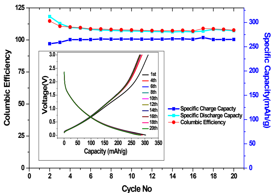
Fig. S1: Li-ion battery cycling performance of pristine carbon nanofibers (without N-doping) (Inset: charge –discharge curve for first 20 cycles)
