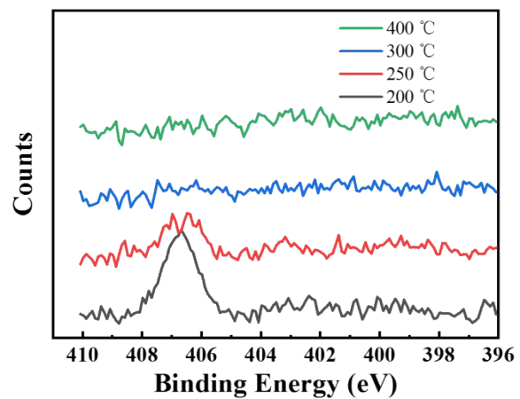
Figure S1. N 1s spectra of ZrO 2 films with different post-annealing temperatures.
