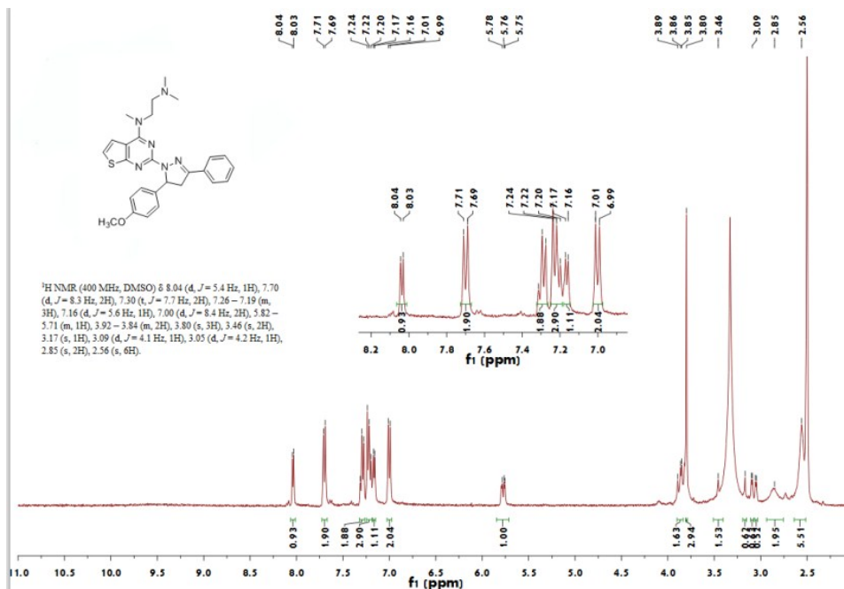
13f. 1 H NMR (400 MHz). Solvent: DMSO
