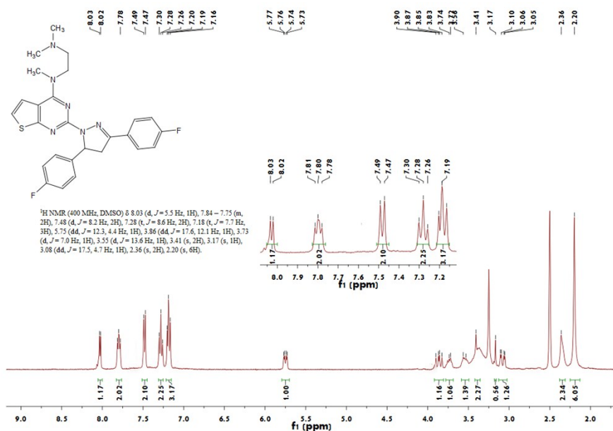
13c. 1 H NMR (400 MHz). Solvent: DMSO
