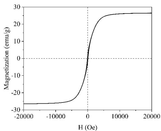
Fig. S1 The magnetic hysteresis curve of Fe/CN@E-3.
