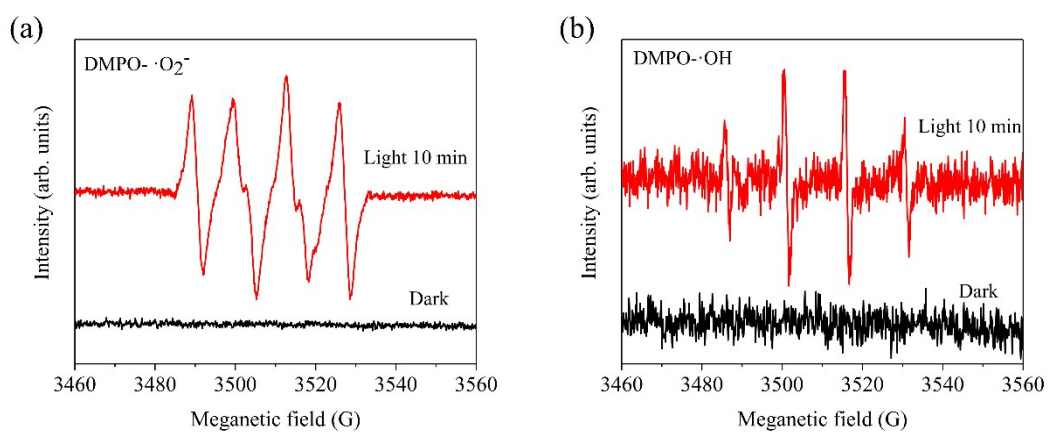
Fig. S2 ESR spectra radicals trapped by DMPO recorded at room temperature under dark and visible light irradiation: (a) DMPO- \cdot\text{O}_2^- response; (b) DMPO- \cdot\text{OH} response.
