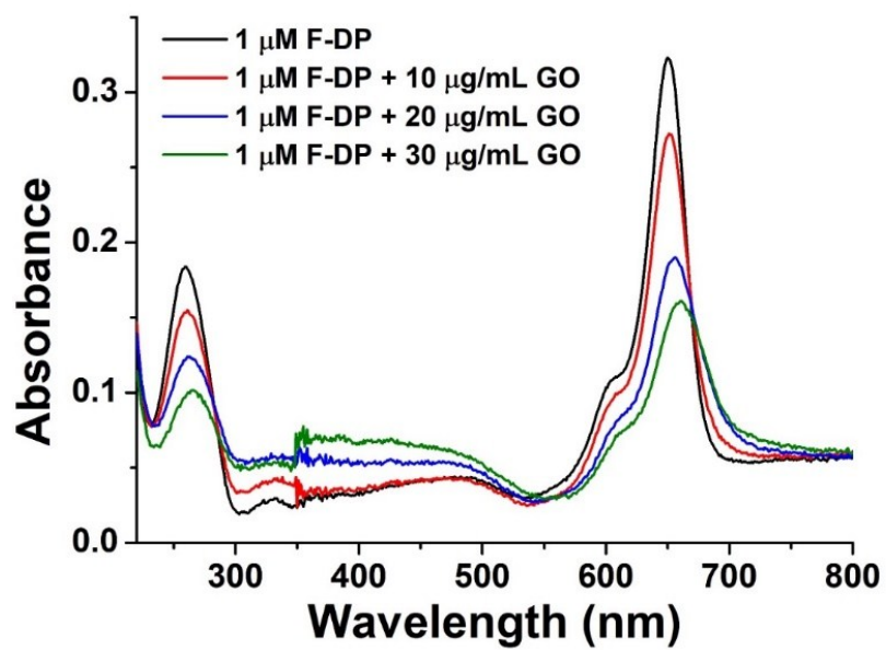
Fig. S1. UV/vis absorption spectra of 1 μM F-DP solutions in the absence and presence of different concentrations of GO.
