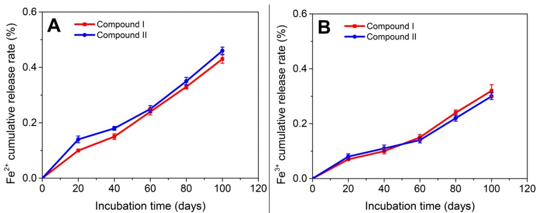
Fig. S2 \text{Fe}^{2+} (A) and \text{Fe}^{3+} (B) cumulative release rates of compounds in water
