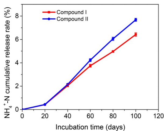
Fig. S1 \text{NH}_4^+\text{-N} cumulative release rate of compounds in water
