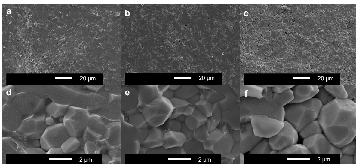
Figure S1: SEM images of the \text{Li}_{7-3x}\text{La}_3\text{Zr}_2\text{Al}_x\text{O}_{12} sintered ceramic at 50 MPa (a,d), 30 MPa (b,e) and 20 MPa (c,f) with two different magnifications.
