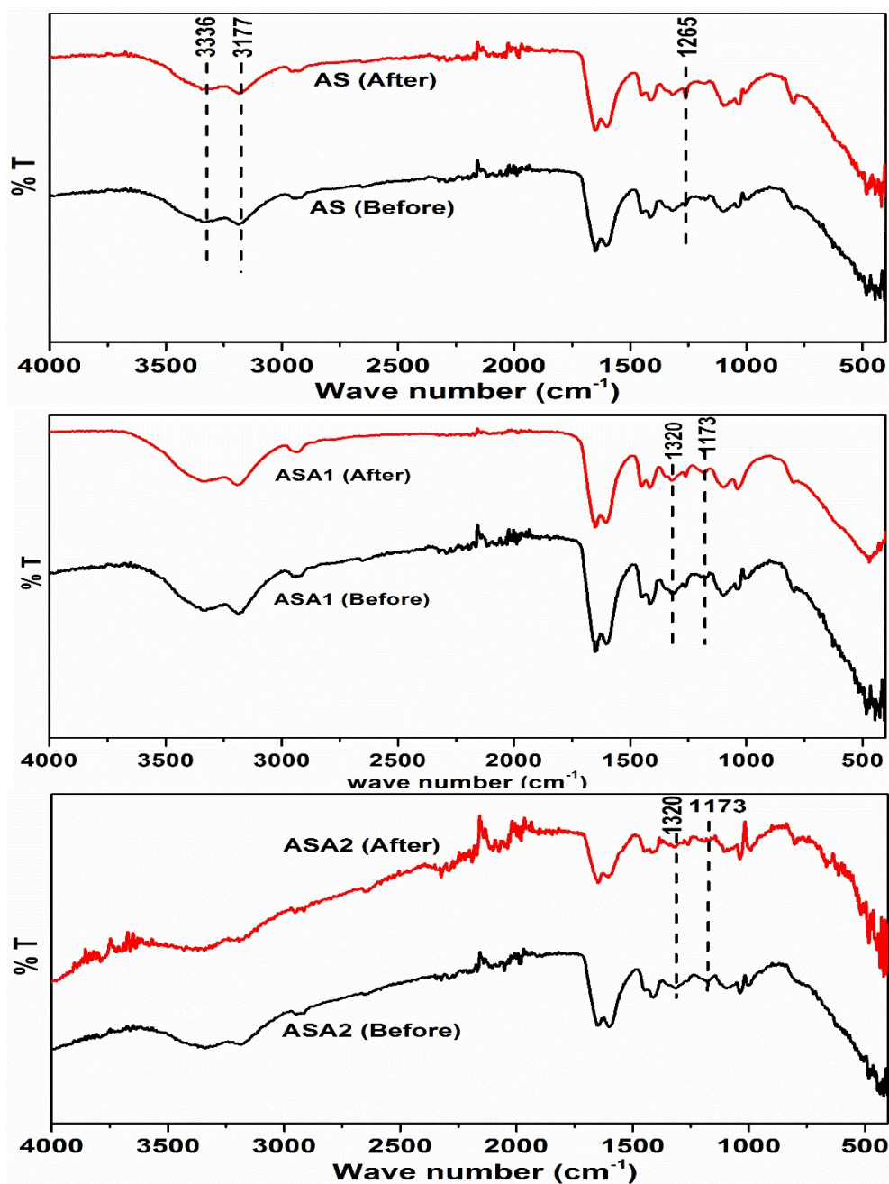
Fig. S1 FTIR spectra for prepared hydrogel samples before and after absorption of CV
