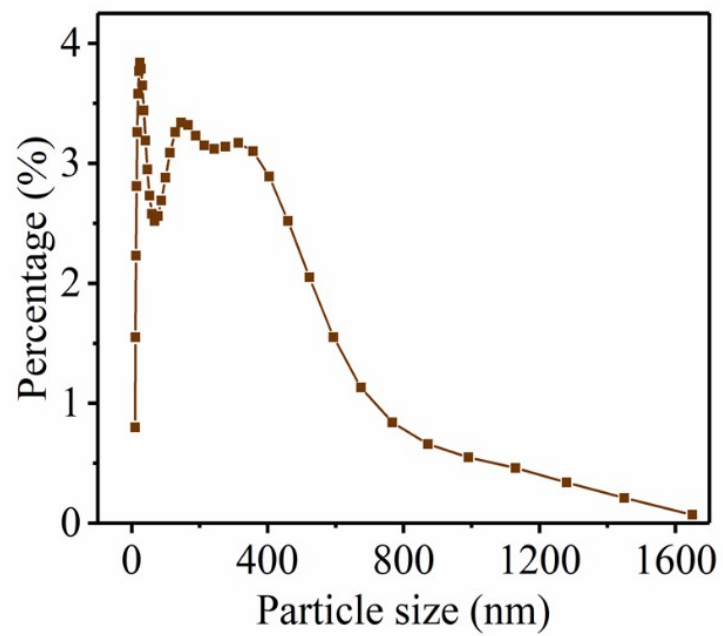
Figure S1 Particle size distribution curve of a commercial Chinese ink
