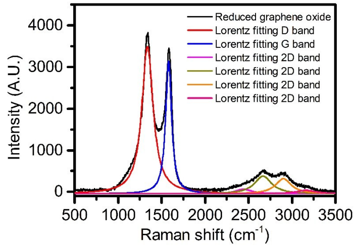
Figure S1. Raman spectrum of the pure Graphene.
