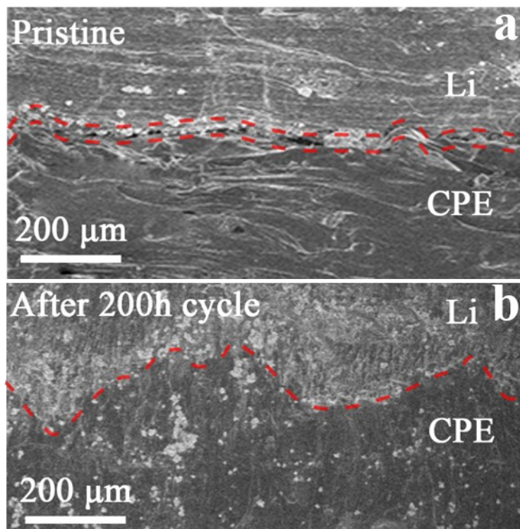
Fig. S1. The cross-sectional SEM images of the lithium metal and CPE before (a) and after 200 hours cycling (b) in the symmetrical cell.
