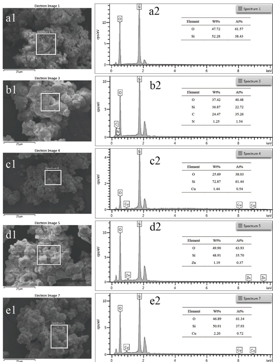
Figure S1. energy dispersive X-ray spectroscopy (EDS) of SBA - 3(a1, a2); G - SBA(b1, b2); SBA/CuO (c1, c2); SBA/ZnO (d1, d2) and SBA/CuZnO (e1, e2)
