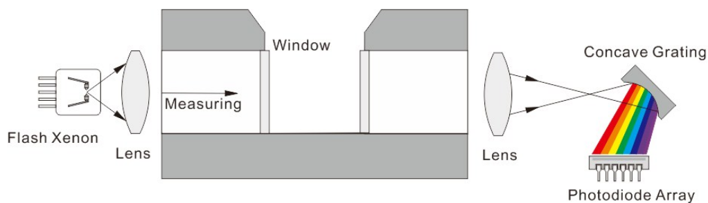
Fig. S2. The schematic diagram of internal structure of developed prototype
