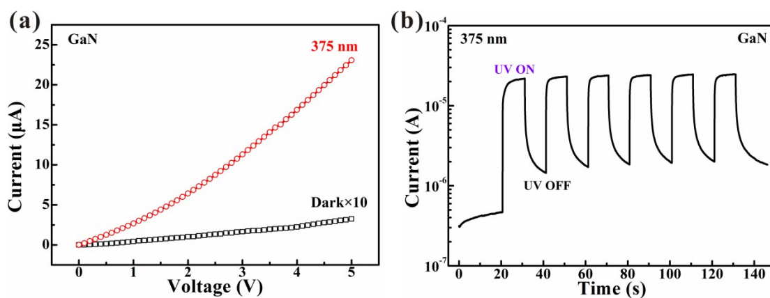
Fig. S1 (a) I-V curves and (b) photoresponse property of GaN substrate.
