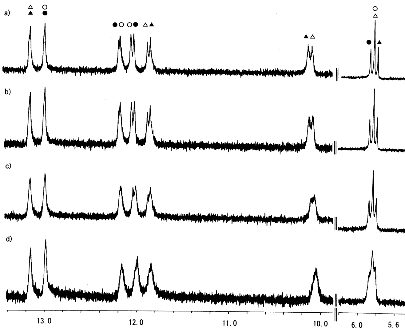
^1\text{H} NMR spectra of a mixture of 2 (4.6 mM) and N -[(butylamino)carbonyl]-6-tridecylisocytosine (UPBu) (4.6 mM) recorded at 500 MHz in \text{CDCl}_3 . a) 298K, b) 303K, c) 313K, d) 323K.
