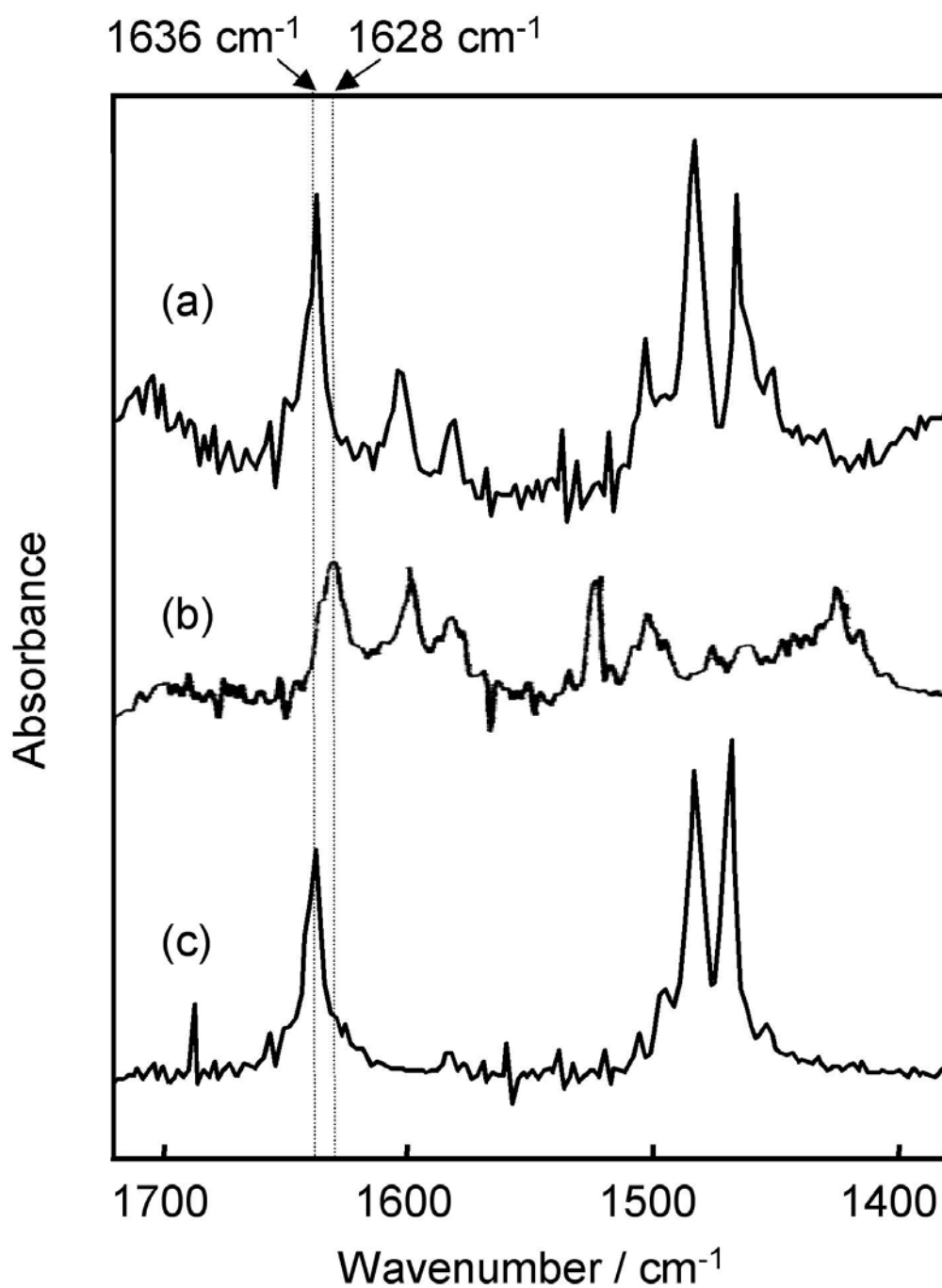
Figure IR spectra of (a) DVB/micelle/silicate composite heated at 110 °C, (b) DVB, and (c) micelle-forming compound (C 16 PyCl).
