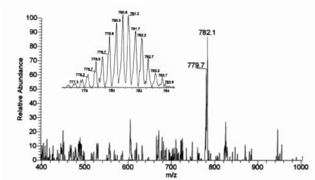
ESI-MS spectra of compound 2
