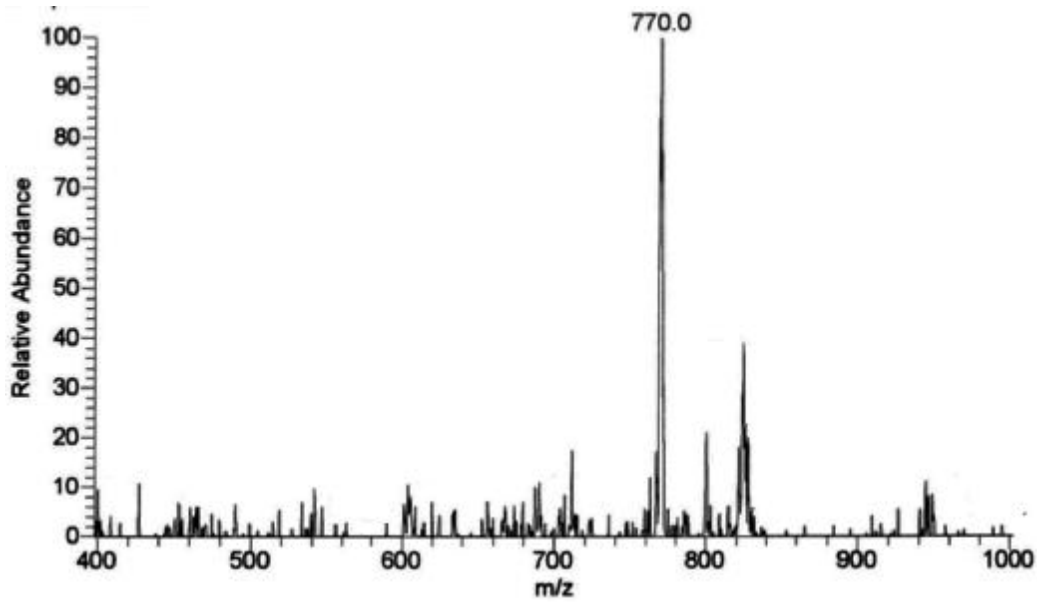
ESI-MS spectra of compound 1
