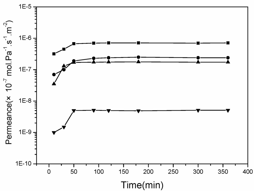
Figure 4 Time dependence of the CO 2 permeation (■, unseeded membrane; ●, seeded membrane) and N 2 permeation (▲, unseeded membrane; ▼, seeded membrane) at the dry temperature of 120°C.
