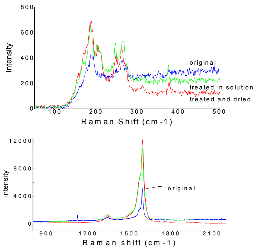
Fig.2 Raman spectra of SWNTs before and after applying the debundling treatment; the top spectra shows the RBM region and the lower spectra shows the G and D peaks. (Key: Blue line: original sample prior to treatment; Green line: treated sample in ethanol; Red line: treated sample dried in a vacuum.)
