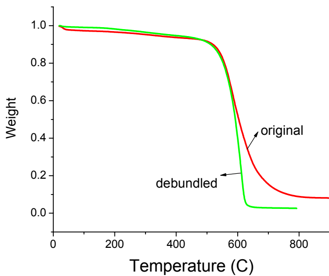
Fig.1 TGA curves of the SWNTs before (red) and after (green) the debundling treatment
