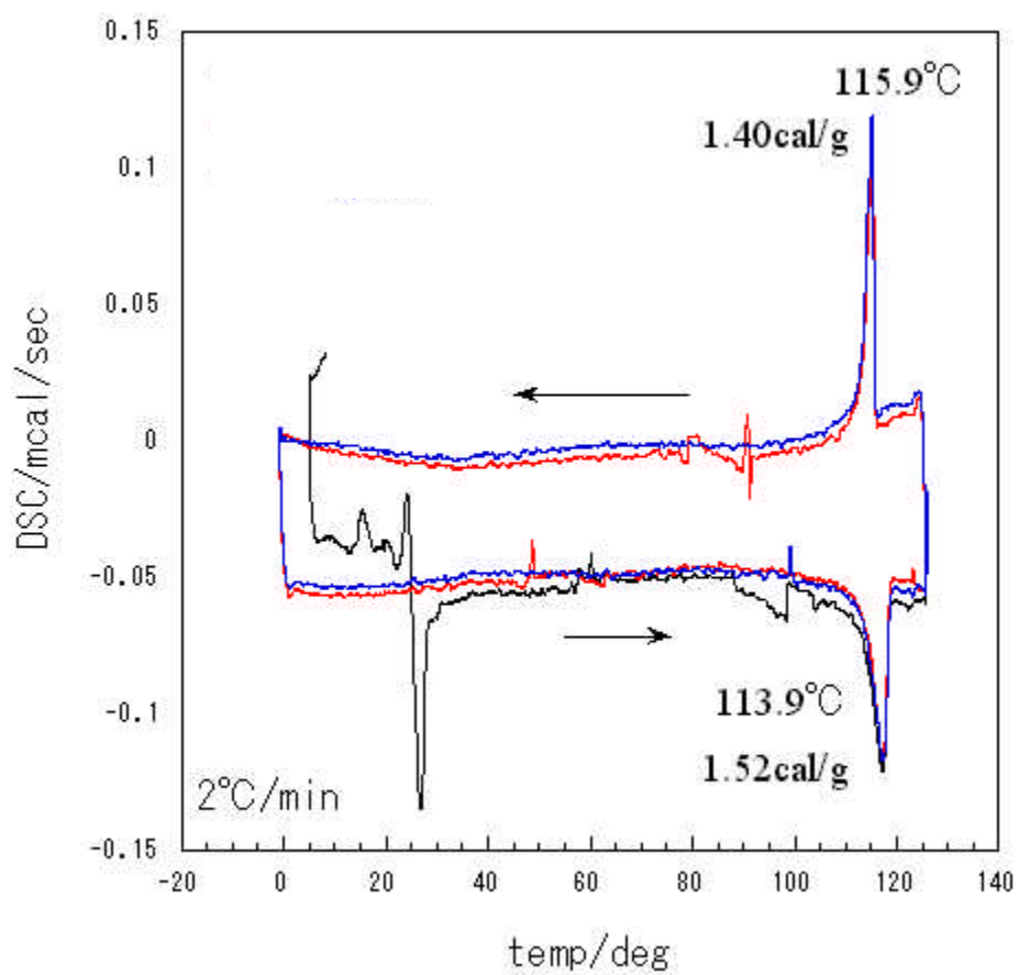
DSC thermogram displayed sharp transitions both on heating and cooling for Col I -I at 115 °C
