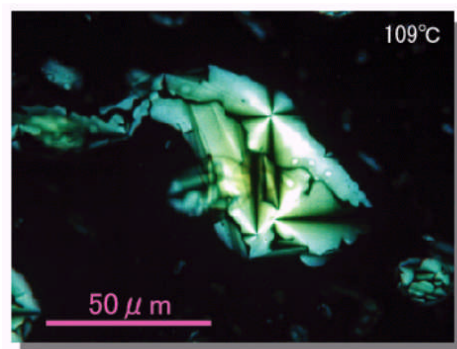
Focal conic fan texture of [Cr(5C 8 ) 3 ] was observed under a polarized light microscope at 109 °C
