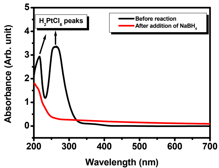
Figure S1. UV absorption spectra before and after the reduction reaction in aqueous \beta -D glucose dispersion (pH = 7.7)
