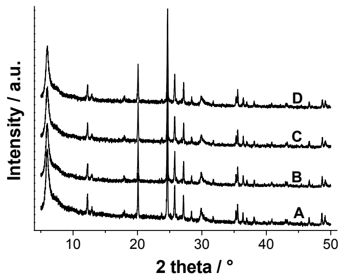
Fig. 1 X-ray powder diffraction patterns of as-made ETS-10 (A) and 10 wt. % H 2 O 2 /ETS-10 (B), 20 wt. % H 2 O 2 /ETS-10 (C), 30 wt. % H 2 O 2 /ETS-10 (D) samples treated under microwave irradiation.
