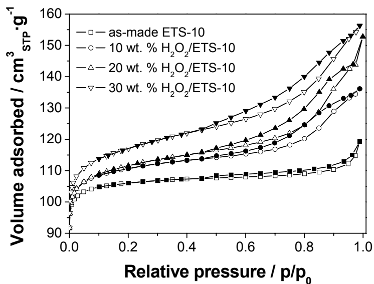
Fig. 2 Nitrogen adsorption/desorption isotherms of as-made and treated ETS-10 samples.
