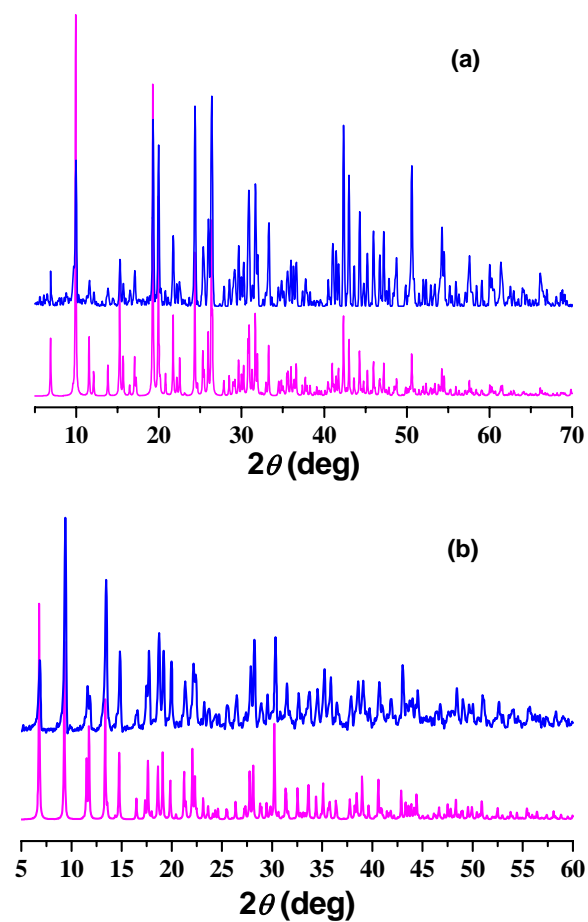
Fig. S1 Observed (blue) and calculated (purple) powder X-ray diffraction patterns for 1 (a) and 2 (b).
