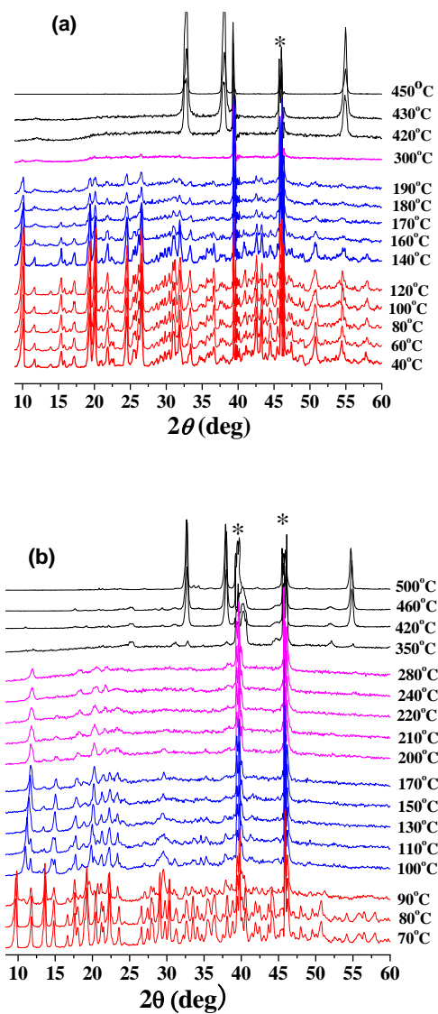
Fig. S3 Variable-temperature XRPD patterns for 1(a) and 2 (b) (*The diffraction peaks of Pt disk).
