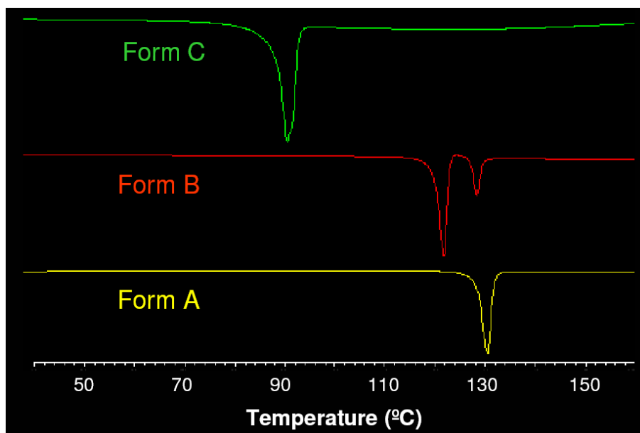
Figure 4. DSC curves of forms A, B and C recorded at 10°C/min. These thermograms show melting of forms A and C, whereas form B melts with crystallization of form A.
