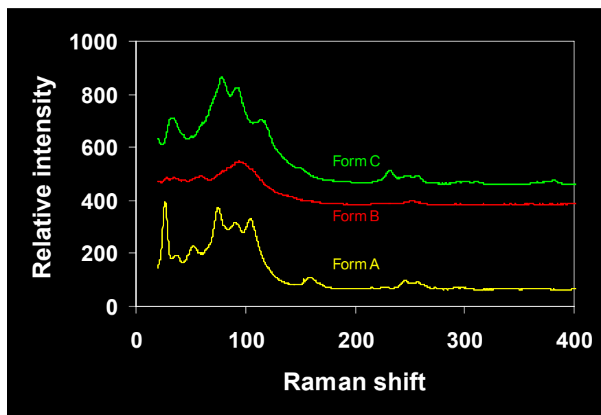
Figure 1. Raman spectra of forms A, B and C.
