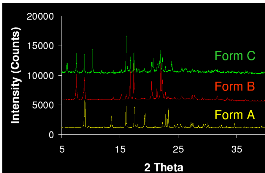
Figure 3. X-ray powder diffraction patterns of forms A, B and C.
