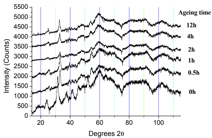
Figure 3: Powder X-Ray diffraction studies of 5%Co/CuMnO x catalyst precursors prepared with a range of ageing times
