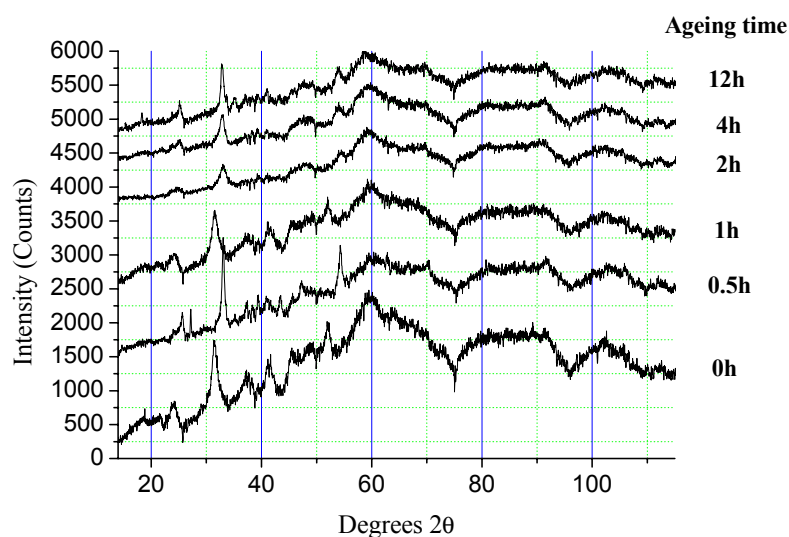
Figure 2: Powder X-Ray diffraction studies of 1%Co/CuMnO x catalyst precursors prepared with a range of ageing times
