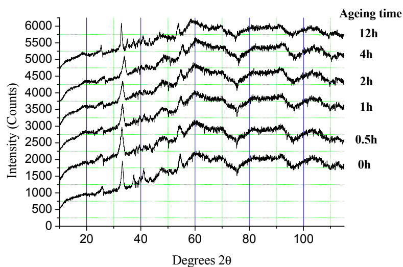
Figure 1: Powder X-Ray diffraction studies of CuMnO x catalyst precursors prepared with a range of ageing times
