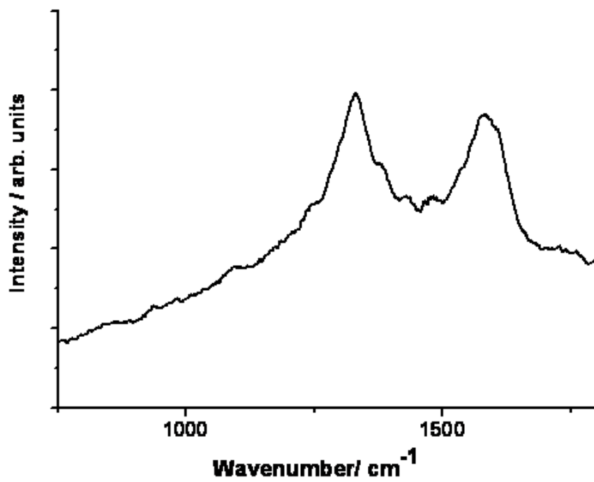
Fig. S2 Raman spectra of thin film of MWCNTs on the PET
