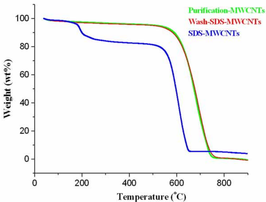
Fig. S2. TGA profile for MWCNTs
