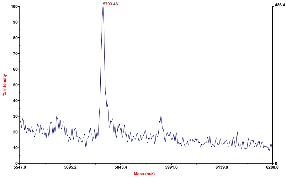
Voyager Spec #1=>NF0.7=>NF0.7=>SM5=>SM5=>AdvBC(23,0.5,0.1)[BP = 5176.8, 16563]
