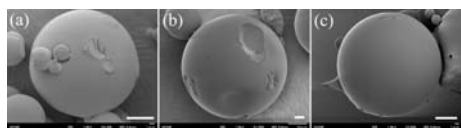
Fig. S1: SEM surface observations of microspheres prepared under the following different conditions: (a) without HAp and NaCl, (b) without HAp but with NaCl, and (c) with HAp but without NaCl”.
