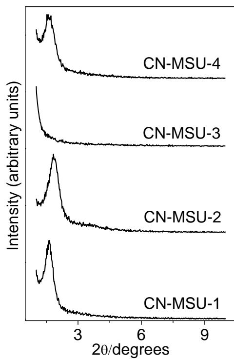
XRD diagrams of CN-MSU-X, X= 1 to 4.
