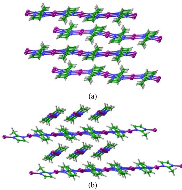
Fig. S4 Crystal packing pattern of 1c viewed along the b -axis (a) and [011] direction (b).
