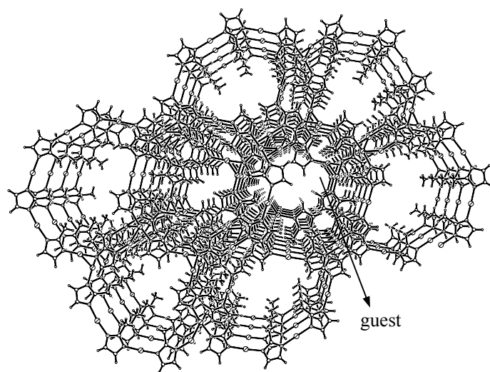
Fig. S2 Crystal packing pattern of 1a viewed along the b -axis.
