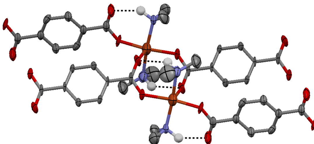
Figure S1. View of 1 with atoms represented as 90 % probability ellipsoids showing the SBU. (H atoms on diethylamine molecules shown as spheres of arbitrary radius; other H atoms not shown).
