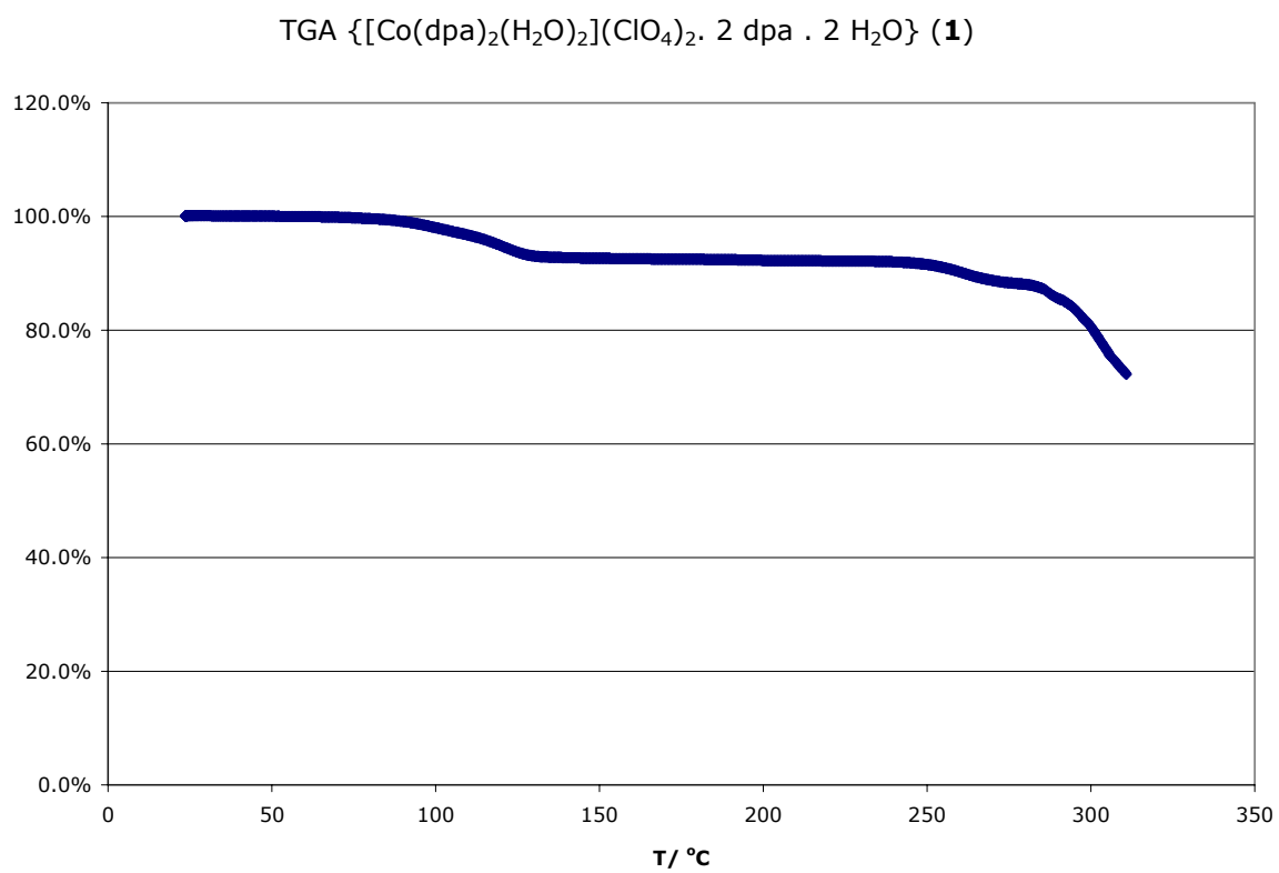
Figure S1. TGA trace for 1 .
