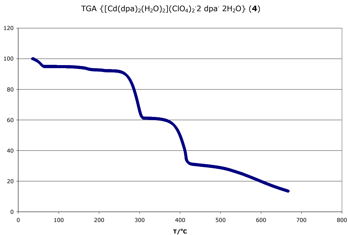
Figure S4. TGA trace for 4 .
