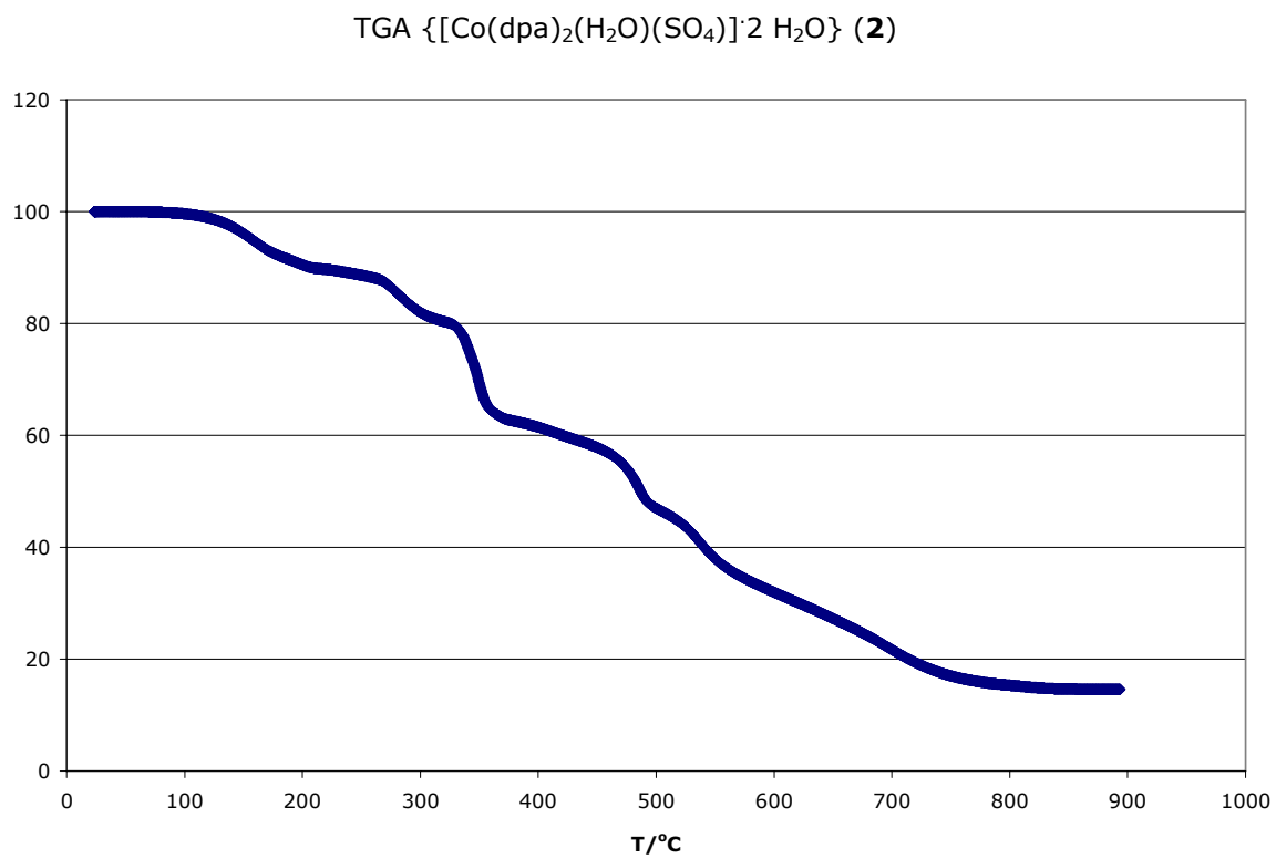
Figure S2. TGA trace for 2 .
