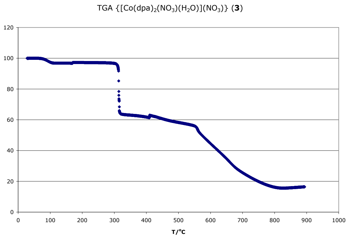
Figure S3. TGA trace for 3 .
