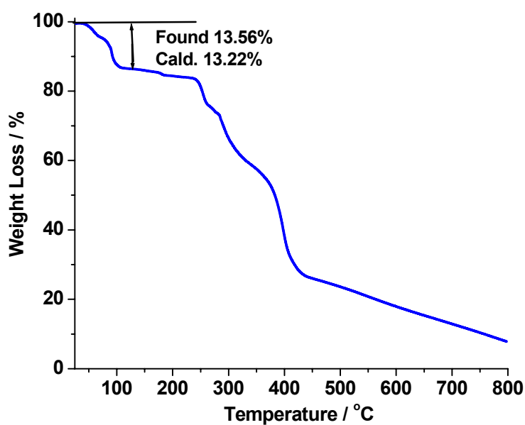
Fig. S2. TGA for compound 1.
