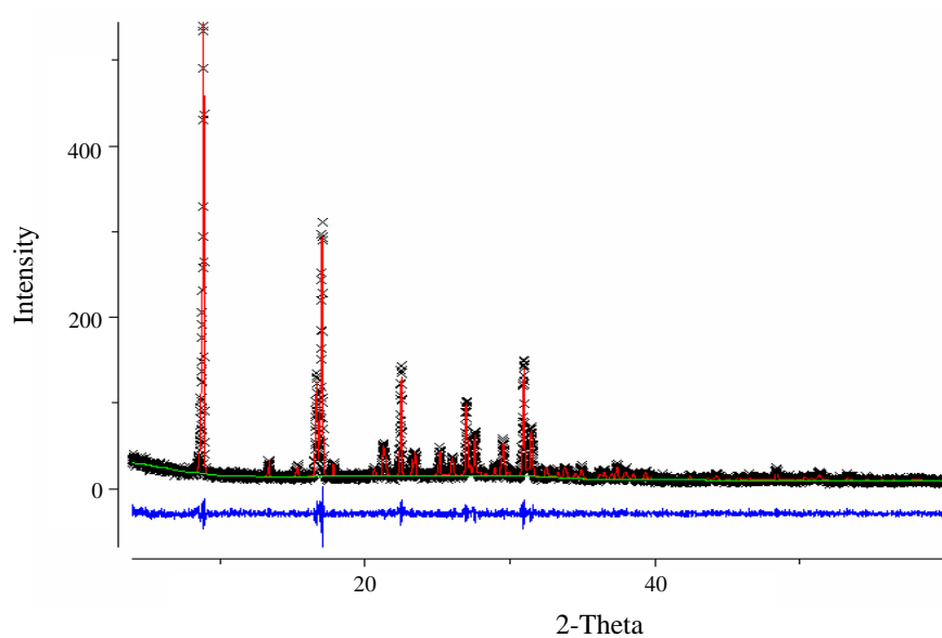
Fig S1 - Rietveld refinement plot 1b . R_{wp} 9.00%, R_{exp} 7.91%. (black) observed, (red) calculated, (green) background, (blue) difference between observed and calculated.
