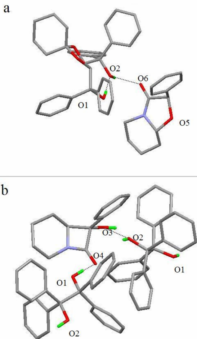
Fig. S2 Compounds (a) I-b'' and (b) V-b'.
