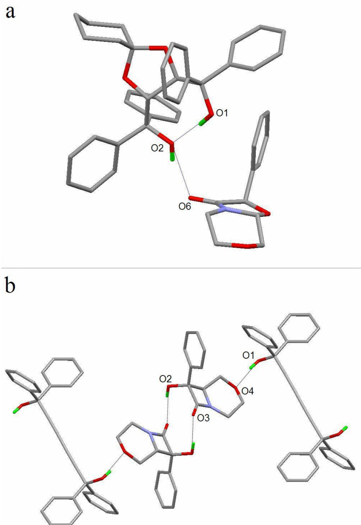
Fig. S1 Hydrogen bonding in inclusion compounds (a) I-a'' and (b) II-a' .
