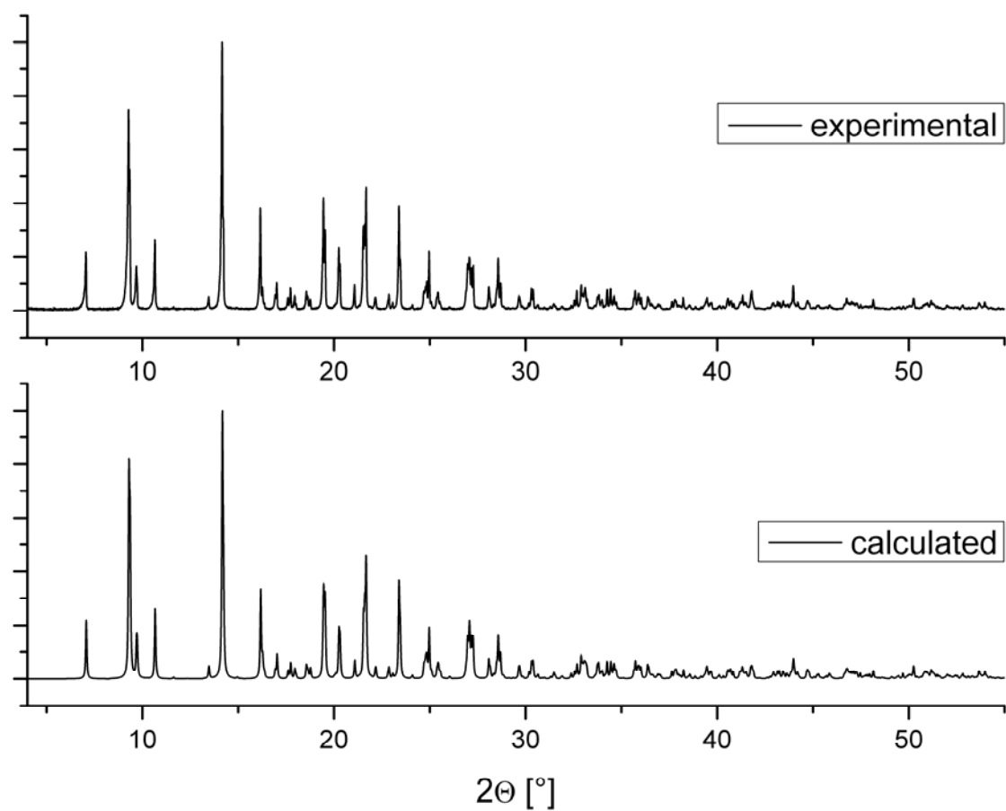
Figure S2 Experimental and calculated powder x-ray diffractograms of 5 .
