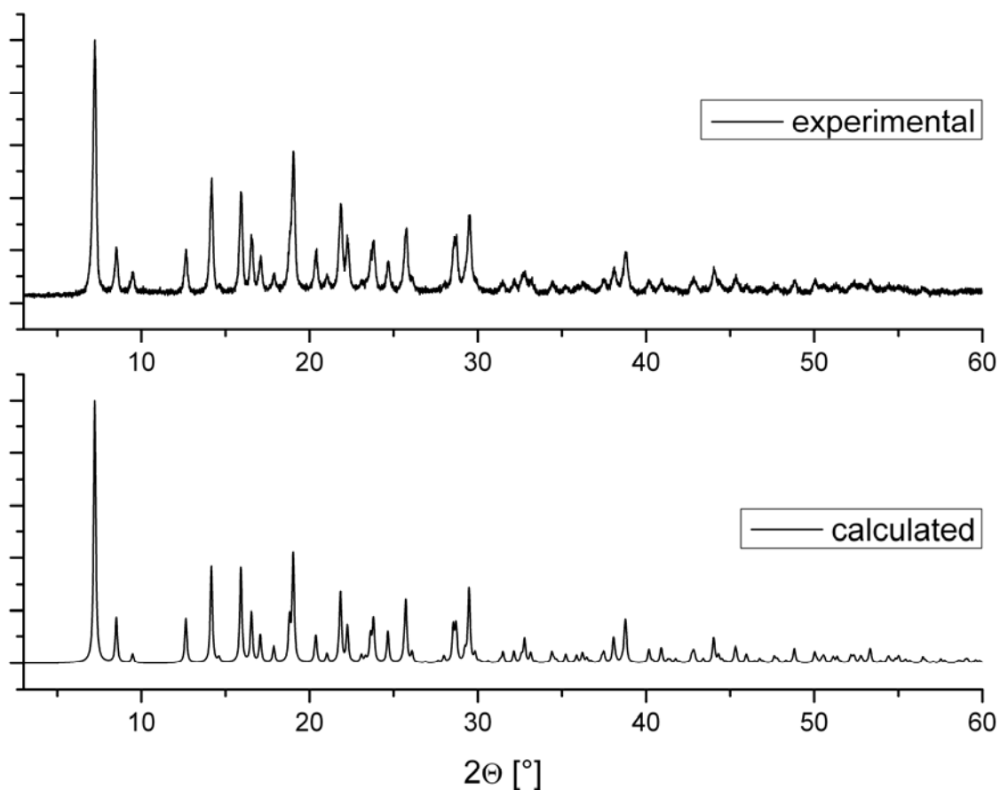
Figure S1 Experimental and calculated powder x-ray diffractograms of 4 .
