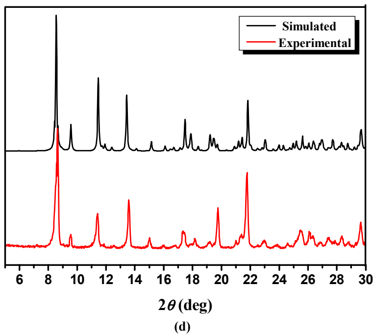
Fig. S4 XRPD patterns for complex 4
