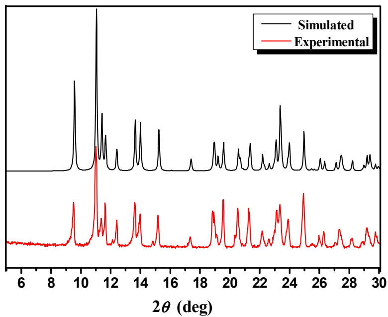
Fig. S3 XRPD patterns for complex 3
