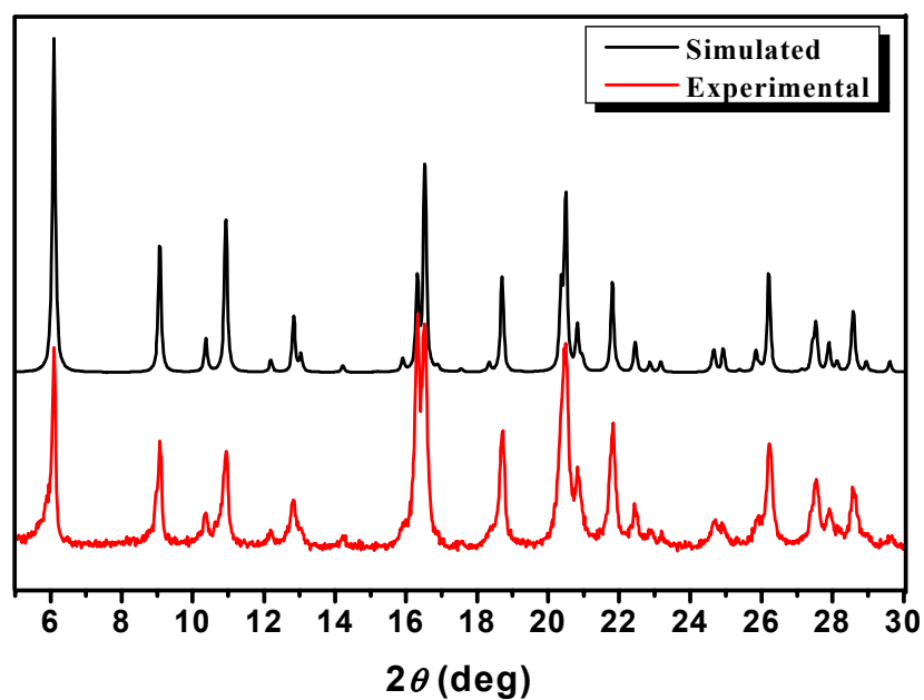
Fig. S1 XRPD patterns for complex 1
