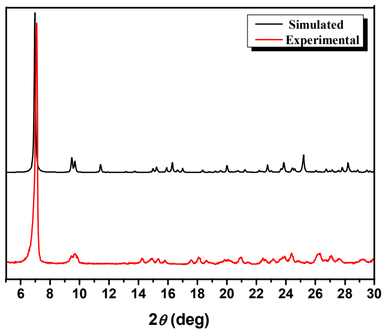
Fig. S2 XRPD patterns for complex 2
